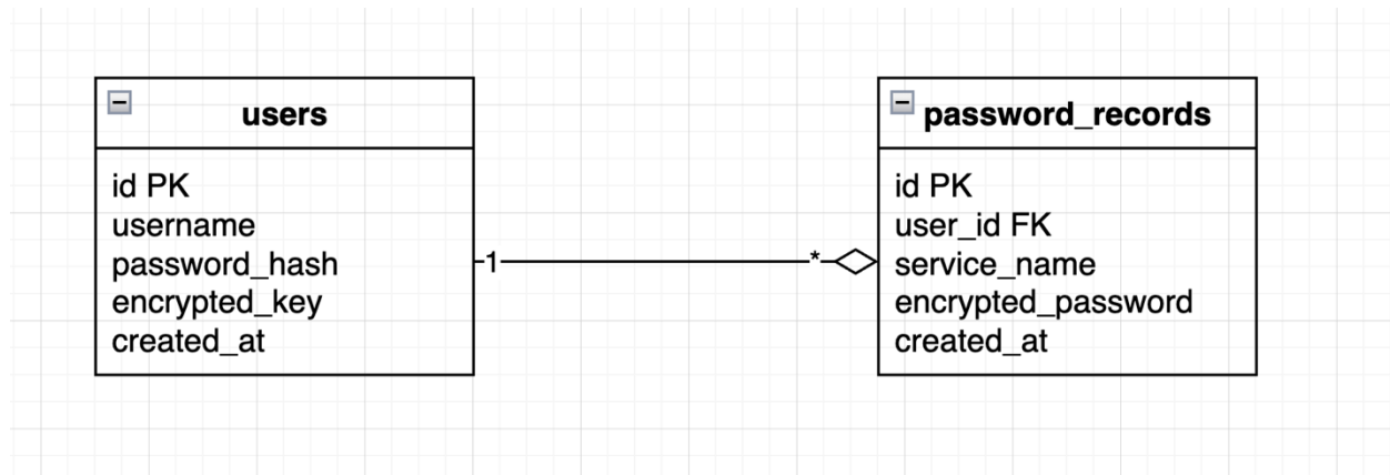
Fig 1: Database
